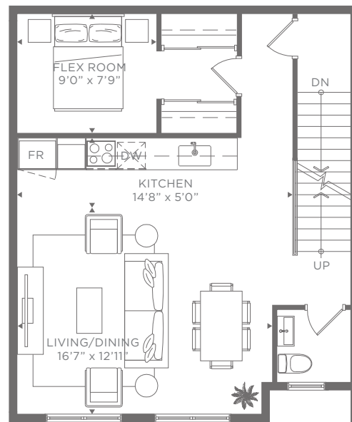
THIRD LEVEL
