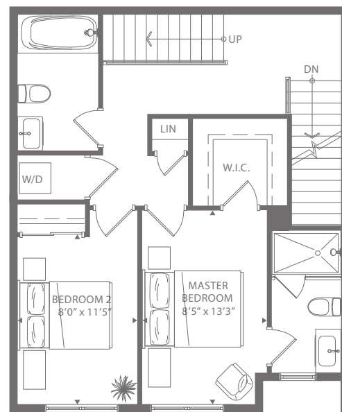
FOURTH LEVEL
