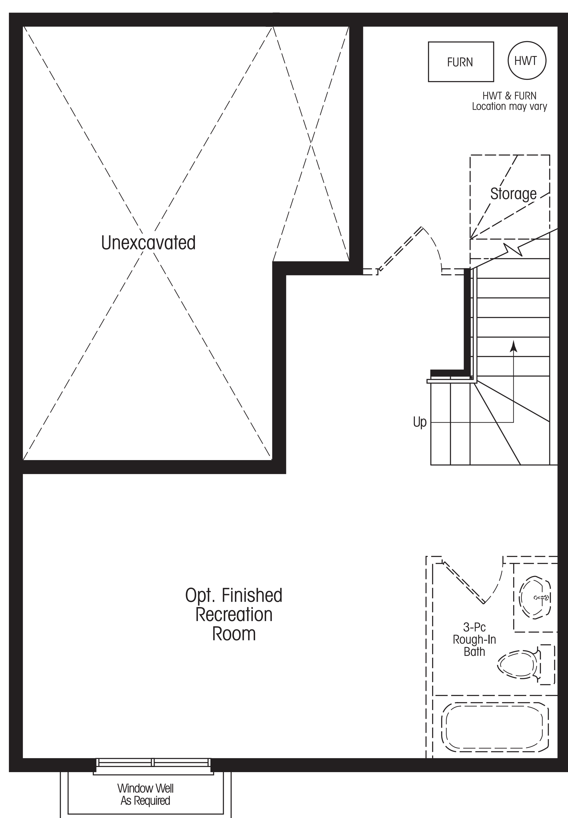
Basement - 471 sf optional finished area
