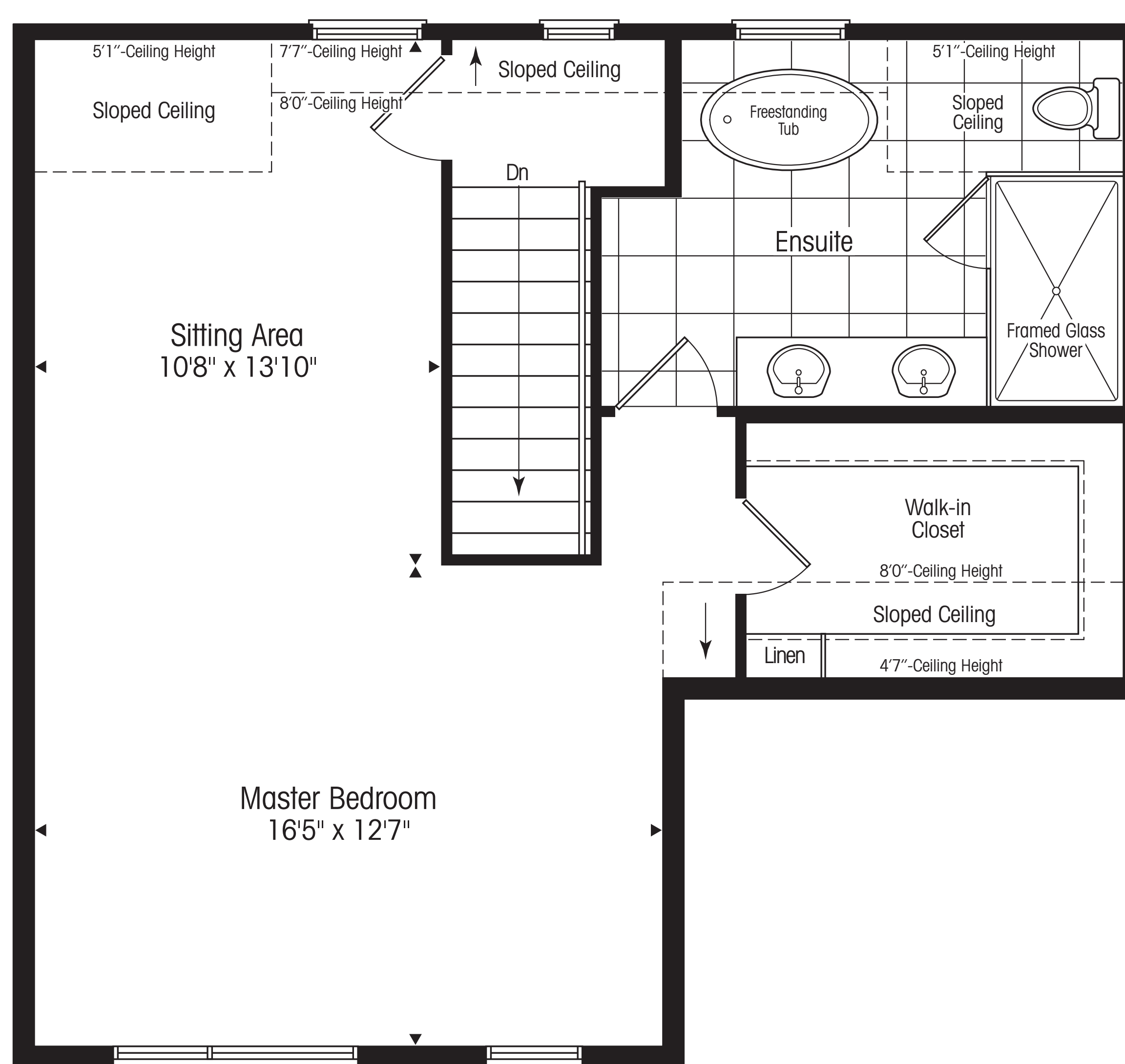
Third Floor - (Lots 11,12) 733 sf
